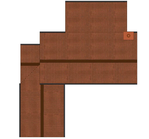
Roof Plan 1:100@A1
