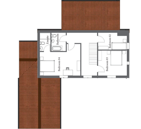
First Floor Plan 1:100@A1
